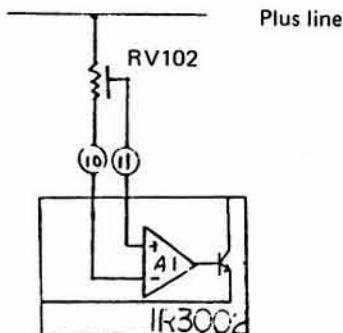
The lock voltage of 2.2 \pm 0.05 V is adjusted by RV102.
